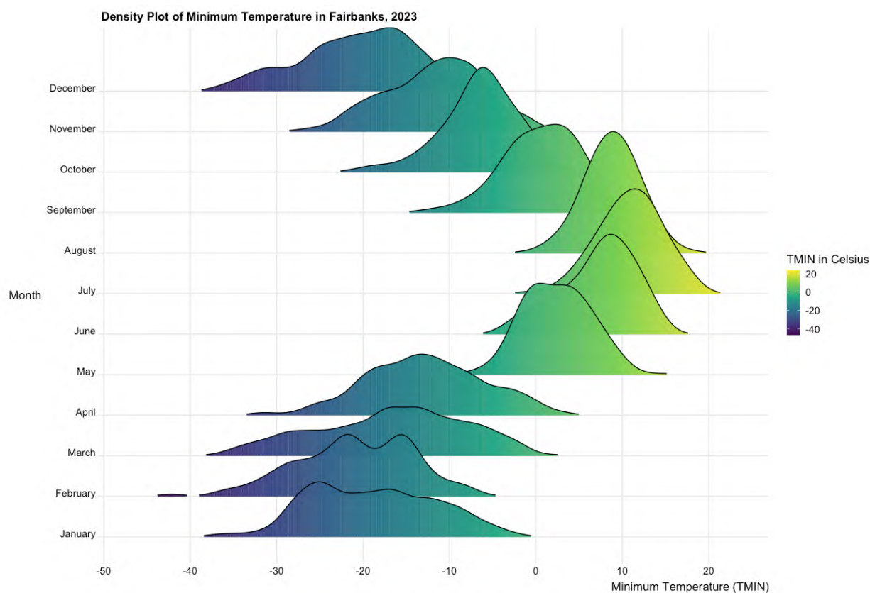
Figure A-4. Minimum Temperature Density in Fairbanks, AK
