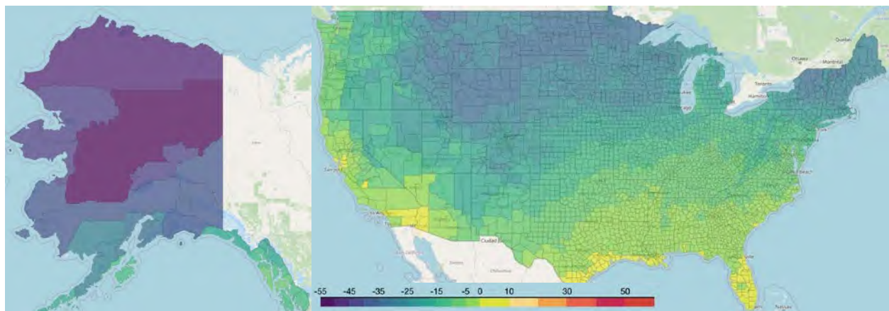
Figure 1. Minimum temperature ( ^{\circ}\text{C} ) reached by U.S. county in 2023
