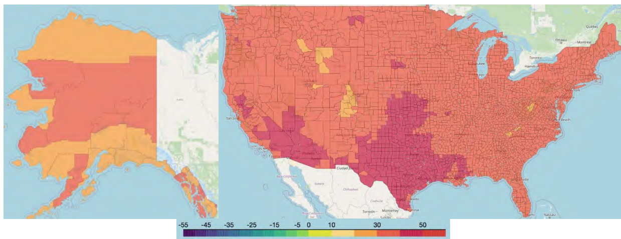
Figure A-3. Maximum daily temperature by county (°C).
