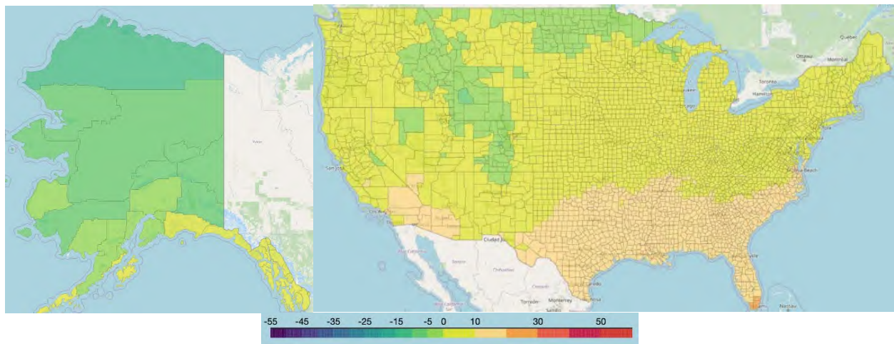
Figure 2. Average minimum temperature ( ^{\circ}\text{C} ) reached by U.S. county in 2023
