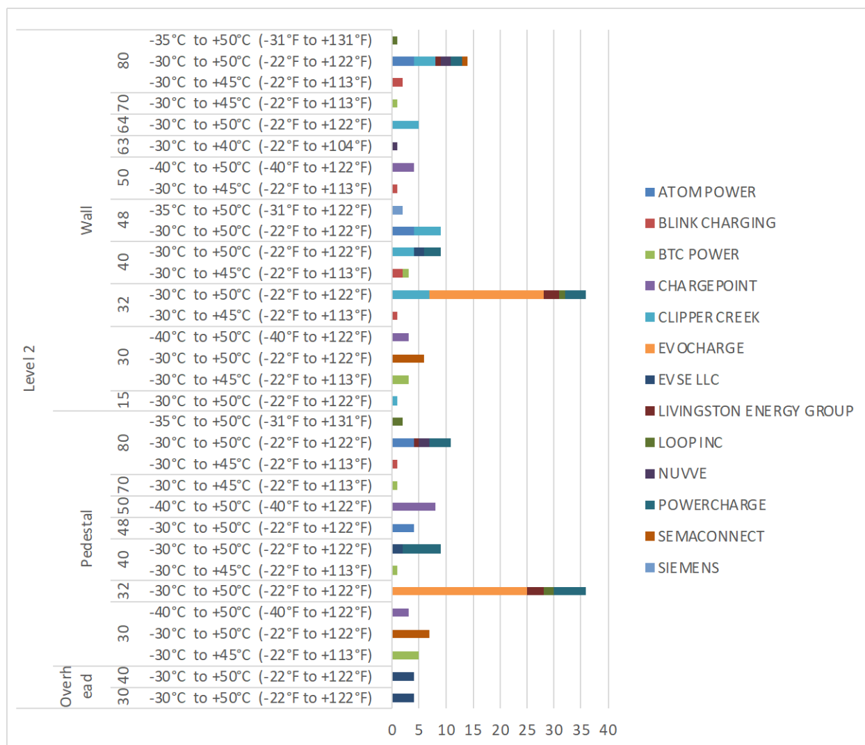
Figure D-1. GSA-available EVSE listed as Level 2, 80-ampere or less power draw, and temperature rating –22°F (–30°C) and below.
