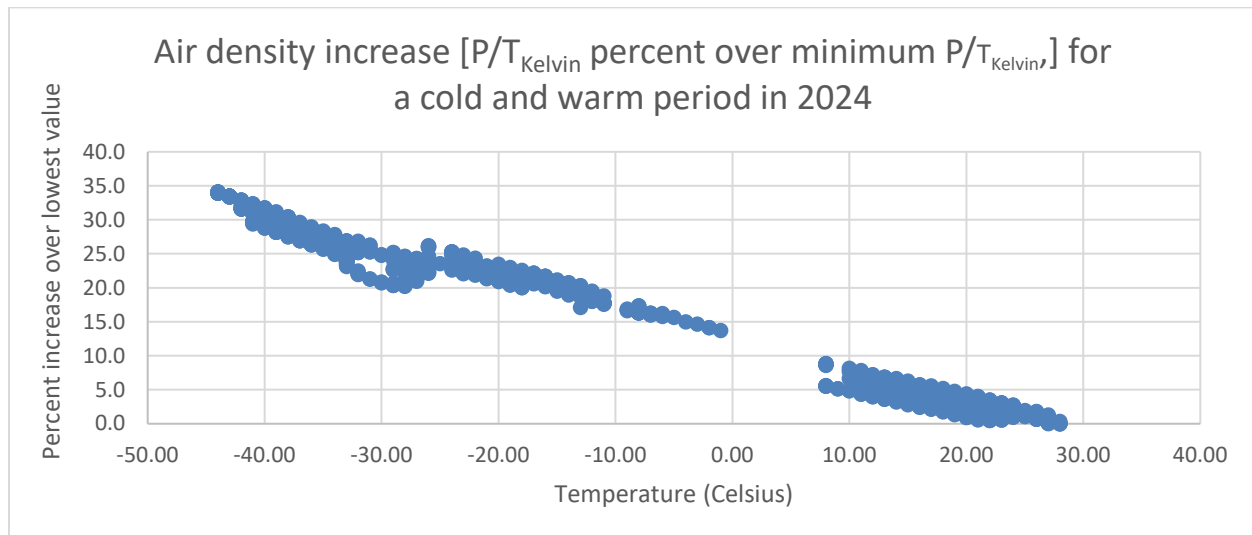
Figure C-1. Air density increase in cold temperatures compared to warm ones.
