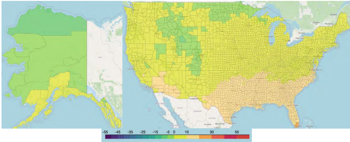
Figure A-1. Average daily temperature by county (°C).
