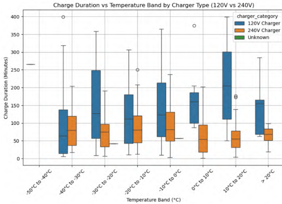
Figure B-1. Charge duration versus temperature by charger type
