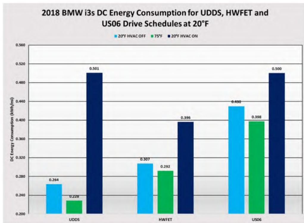
Figure 5. AAA test results for 2018 BMW i3 at 20°F.
