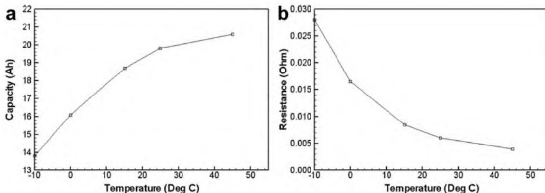
Figure 4. Lithium battery capacity decreases and resistance increase in cold temperatures.
