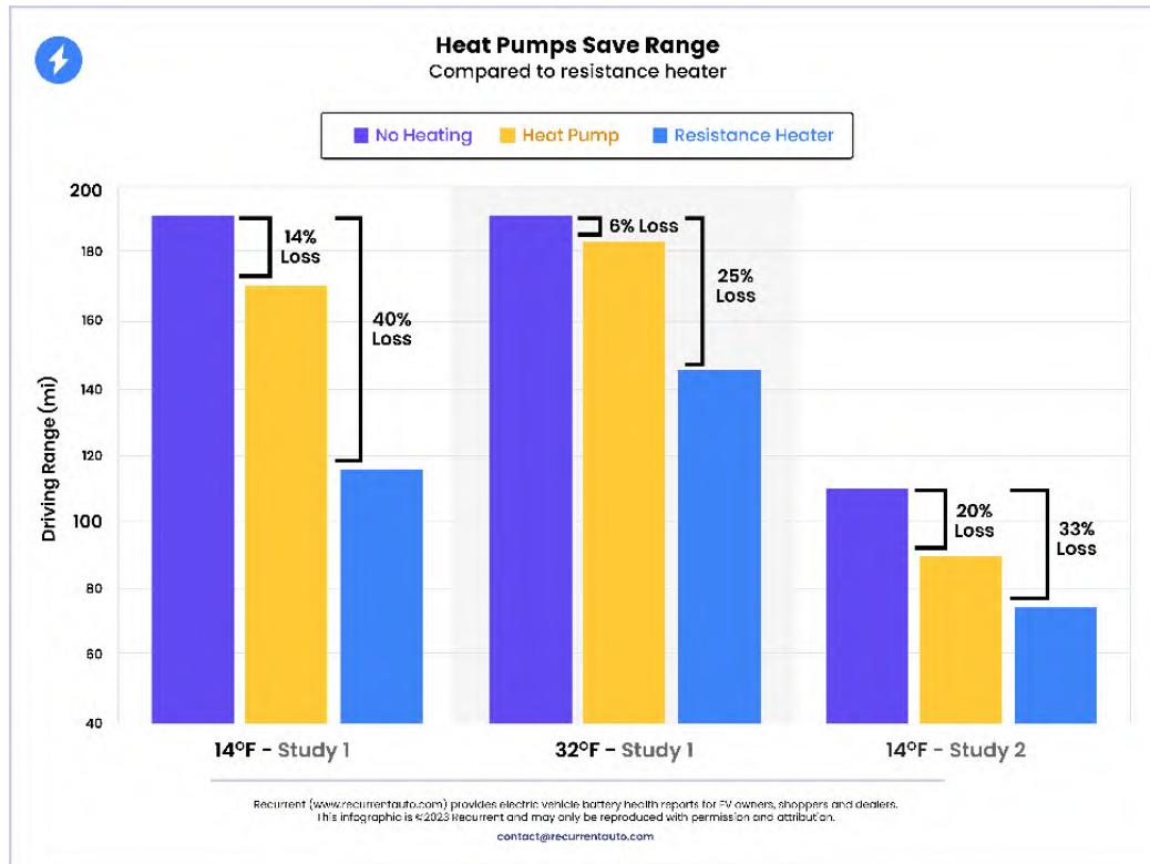
Figure 6. EV driving range difference between heat pumps and resistive heaters.
