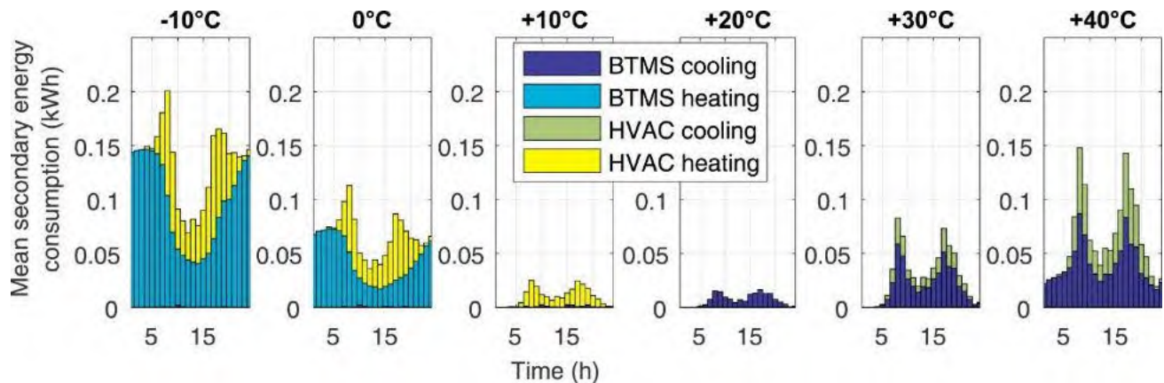
Figure 7. Heating and cooling energy consumption from HVAC and BTMS.
