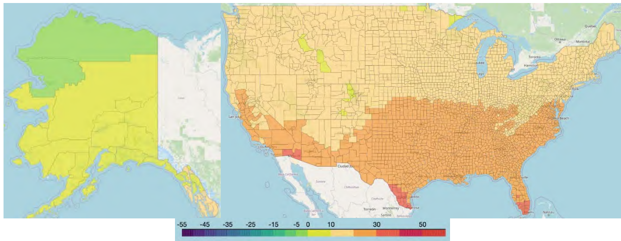
Figure A-2. Average maximum temperature by county (°C).
