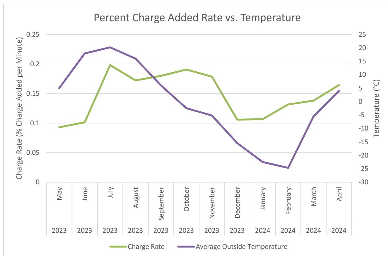
Figure 17. Percent charge added rate versus temperature
