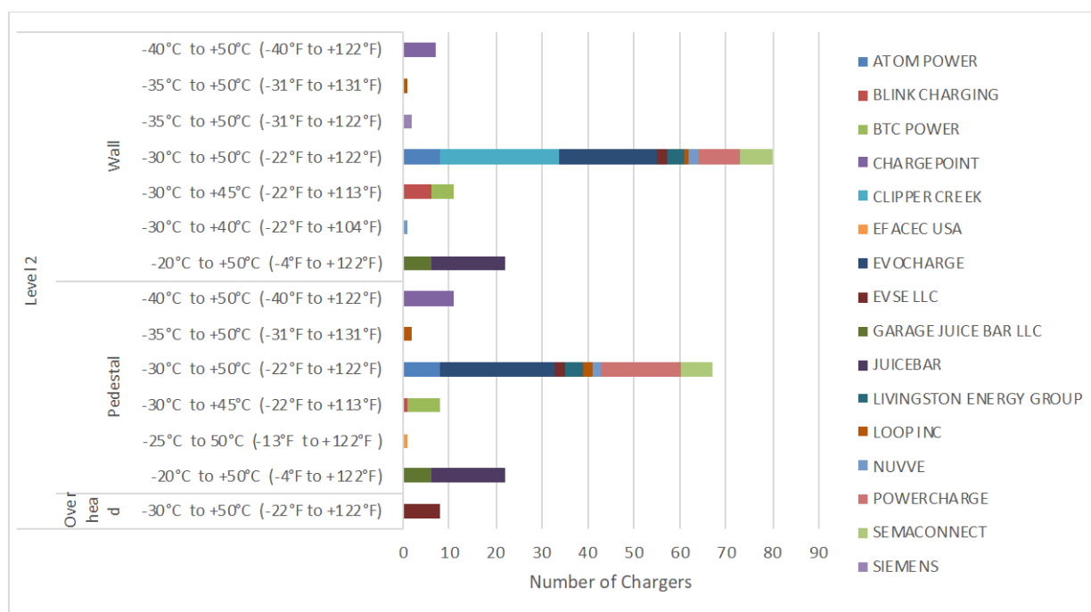
Figure 15. Charging temperature ratings for Level 2 chargers on GSA schedule
