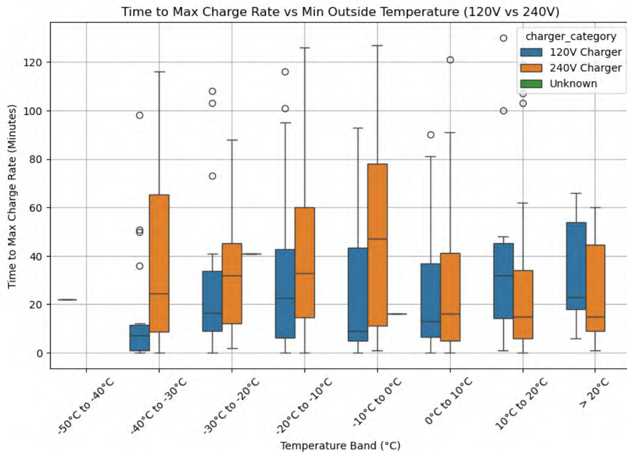
Figure B-3. Time to maximum charge rate versus minimum outside temperature
