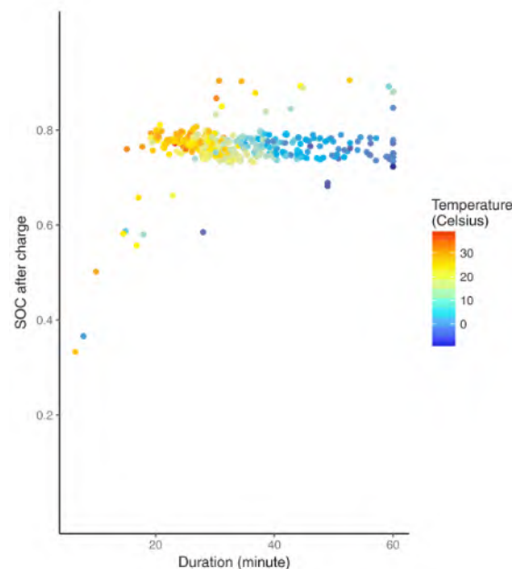
Figure 13. Dependence of DCFC final SoC on temperature.
