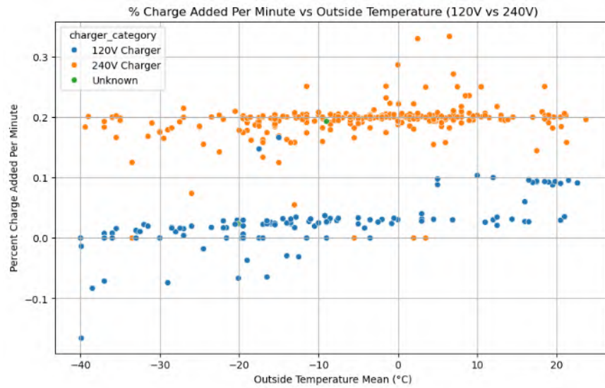
Figure B-2. Percent charge added per minute versus outside temperature
