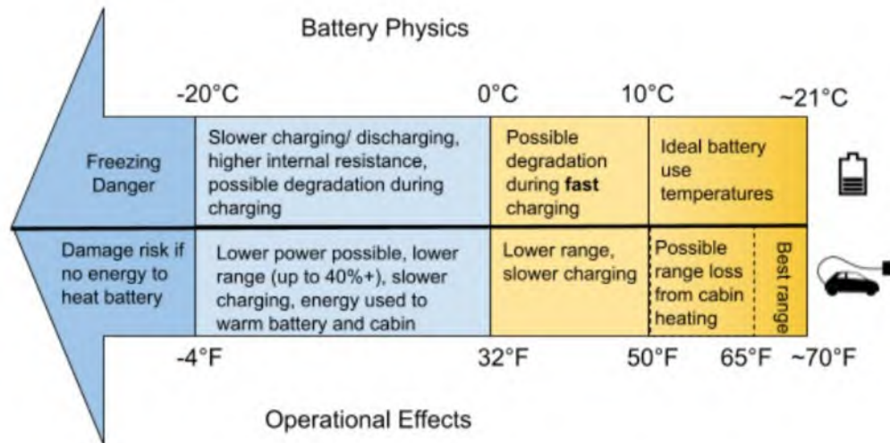
Figure 11. Battery effect (upper portion) and operational effects (lower portion) of cold temperatures on EVs.
