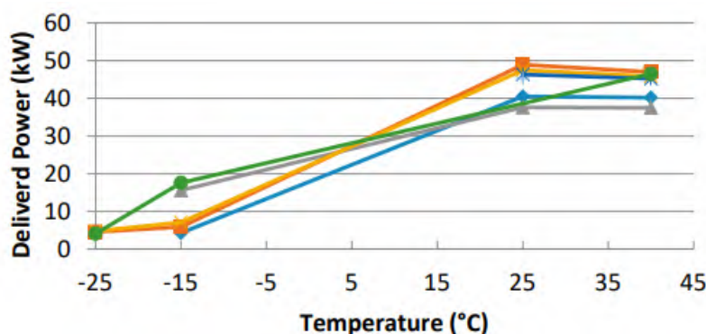
Figure 14. DCFC (i.e., Level 3 charger) delivered power as a function of temperature.
