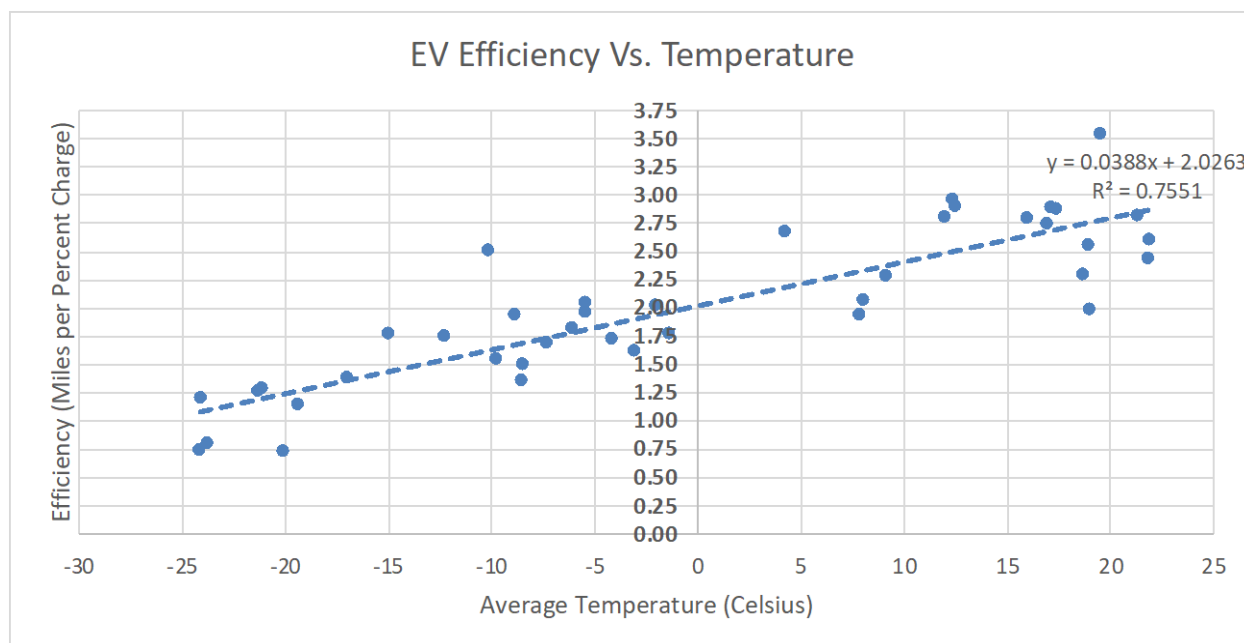
Figure 9. EV efficiency versus temperature for three tesla in Fairbanks, Alaska
