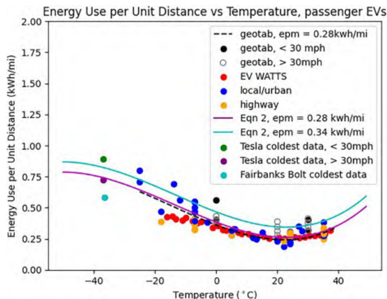
Figure 10. Energy use as a function of temperature, crowdsourced from Alaska EV users.
