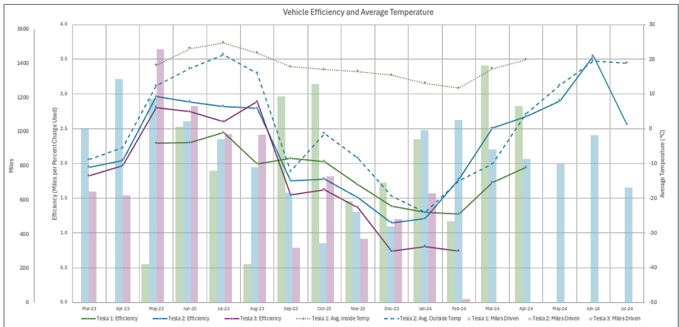
Figure 8. Vehicle efficiency and average temperature
