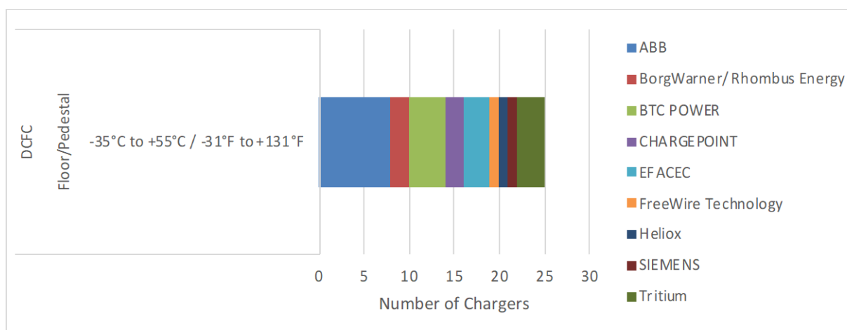
Figure 16. Charging temperature ratings for DC charging on GSA schedule
