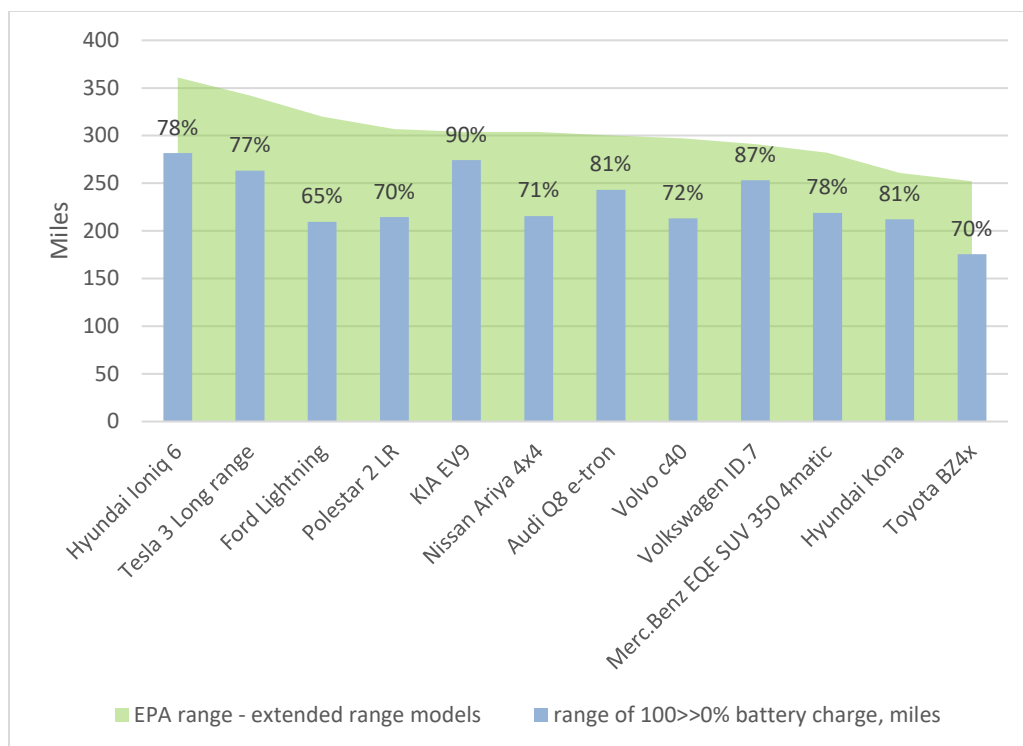
Figure 12. The range (miles) of some EVs tested in Norway at 14°F–28°F weather, in comparison to the stated EPA range for the models.
