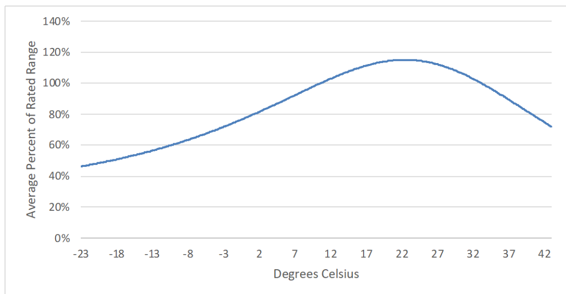
Figure 3. Average EV range as a percentage of rated driving range.
